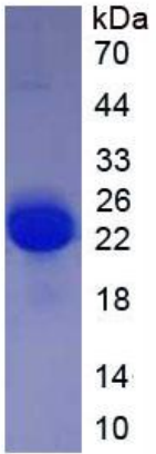
Figure 2. SDS-PAGE
